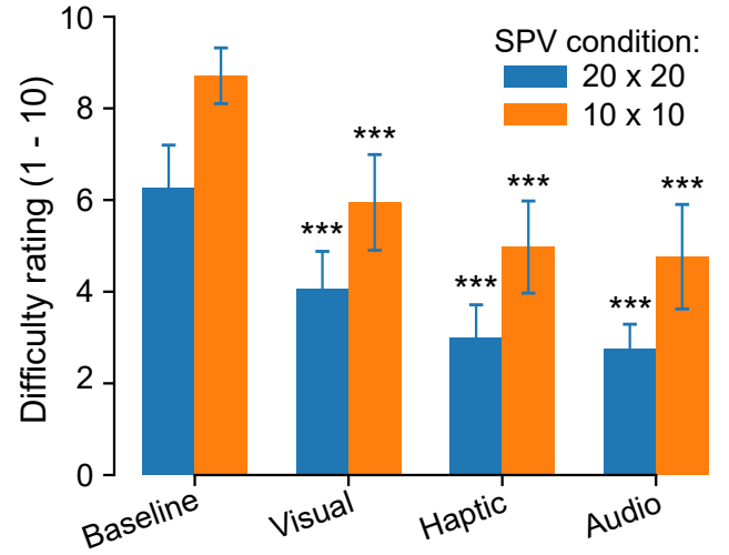
Figure 7: Reported search difficulty by guidance modality and SPV condition. Bars show participant means with 95% confidence intervals; higher scores indicate greater difficulty. Asterisks mark planned within-SPV-condition contrasts against baseline, Holm-corrected within each contrast family ( ***p < .001 ).
